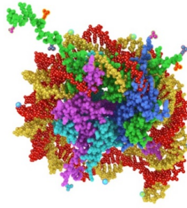
Figure 1 – A nucleosome
